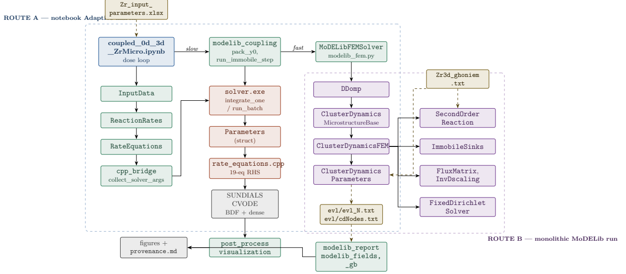
Figure 1: Component call graph. Solid arrows are calls, dashed arrows are file input/output. Blue: orchestrating notebook; green: ZrMicro Python; red: ZrMicro C++; purple: MoDELib3 C++; ochre: files on disk; gray: products. Route A drives the fast mobile solve through MoDELib3 and the slow immobile march through the ZrMicro integrator; Route B runs both inside MoDELib3. The two routes share the material definitions and the post-processing layer.
